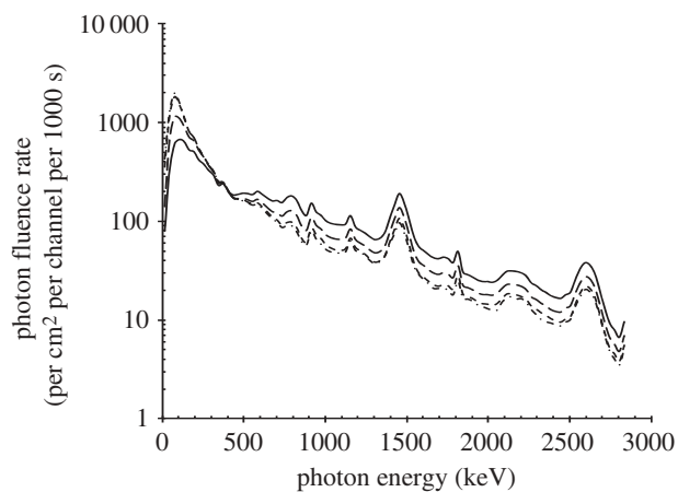
Figure 3. Incident isotropic free-in-air gamma-radiation fluence-rate spectrum, and internal photon fluence-rate spectra. Solid line, incident outside body; long-dashed line, just inside body; small-dashed line, half-way inside body; dashed-dotted line, on axis inside body.
