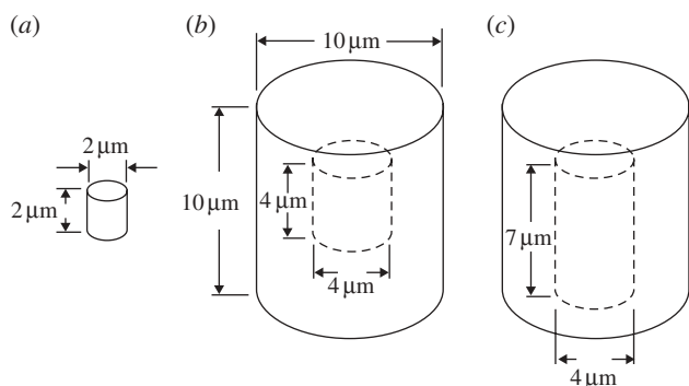
Figure 5. Particle models. (a) Small solid particle. (b) Large particle with closed cavity. (c) Large particle with open cavity. These particles are made of uranium and are surrounded by, and the cavities filled with, ICRU four-element tissue. Particle (c) has the same outer dimensions as particle (b). The closed cavity in particle (b) is centrally located within that particle. The open cavity in particle (c) opens at the bottom of the particle shown.
